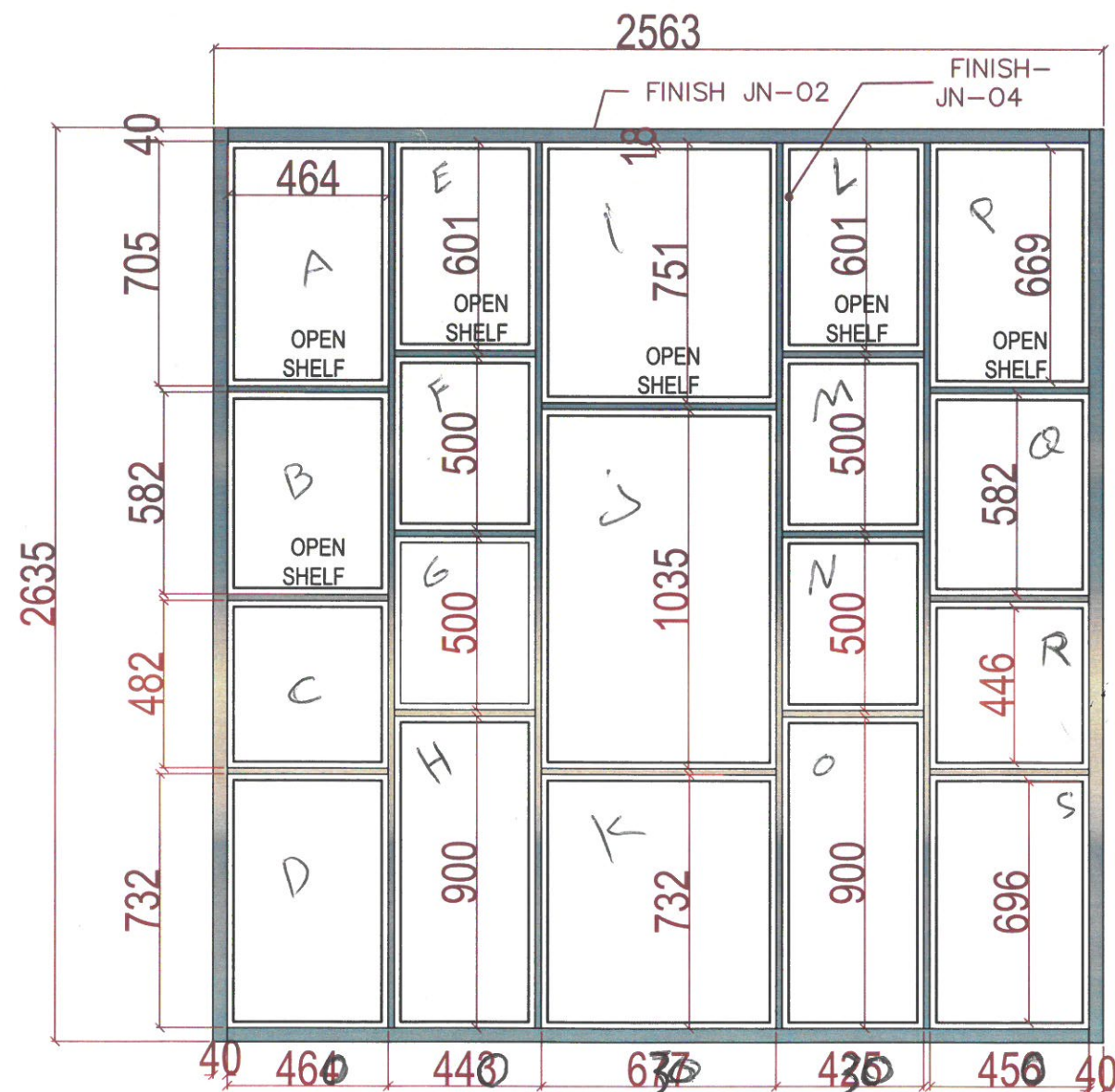
FRONT VIEW FAMILY LOUNGE -DISPLAY SHELF
